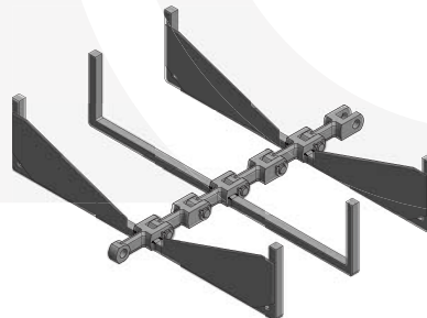
"U" scraper for inclined transport
